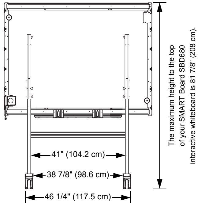
Floor Stand-Mounted Back View (Highest Position)
