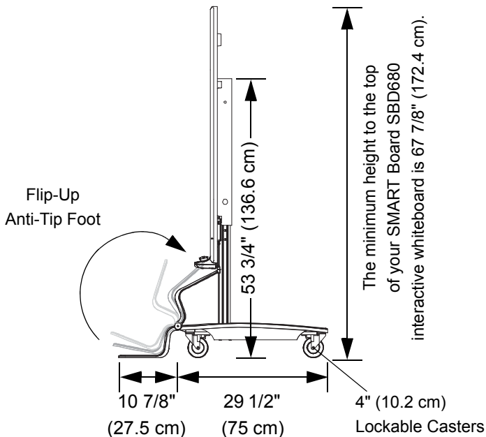
Floor Stand-Mounted Side View (Lowest Position)
